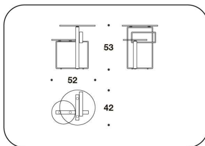
TCT (CA24A) SIDE TABLE 52x42x53H.cm 20 1/3x16 2/4x21H."
