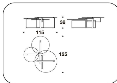
TCT (CA25) COFFEE TABLE 115x125x38H.cm 45 1/3x49 1/3x15H."
