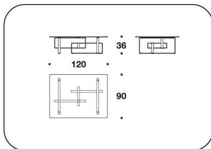
TCT (CA29) COFFEE TABLE 120x90x36H.cm 47 1/3x35 1/3x14 1/4H."
